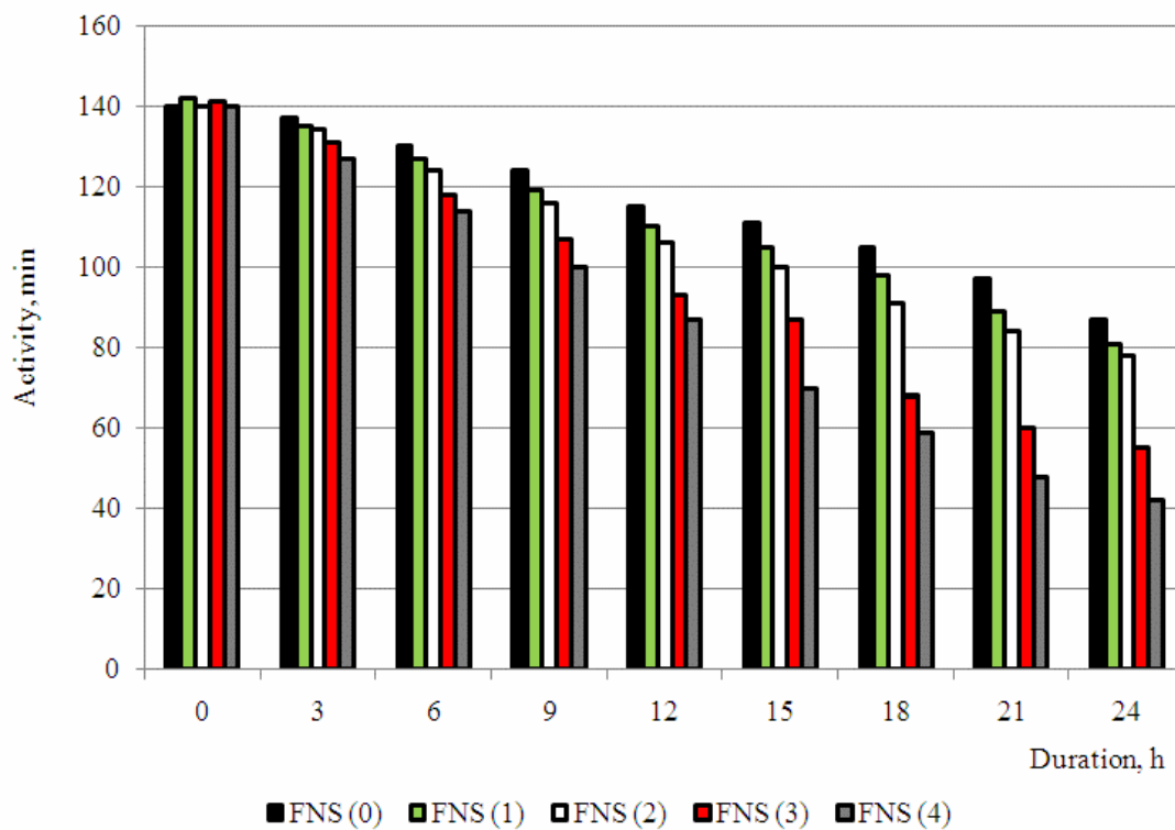
Figure 3. The change in the activity of microorganisms from bacterial concentrate "LBC" depending on the composition of flour nutrient substrates and the duration of cultivation of microorganisms
