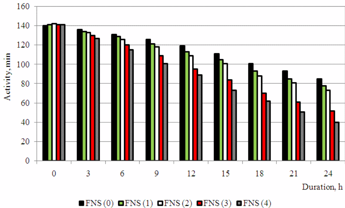
Figure 2. The change in the activity of microorganisms from bacterial concentrate "TV-M" depending on the composition of flour nutrient substrates and the duration of cultivation of microorganisms
