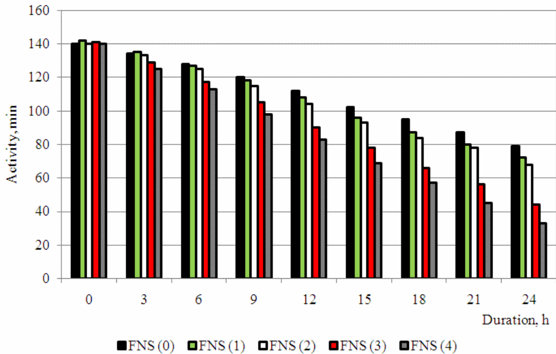
Figure 1. The change in the activity of microorganisms from bacterial concentrate "IM-pro 1" depending on the composition of flour nutrient substrates and the duration of cultivation of microorganisms
