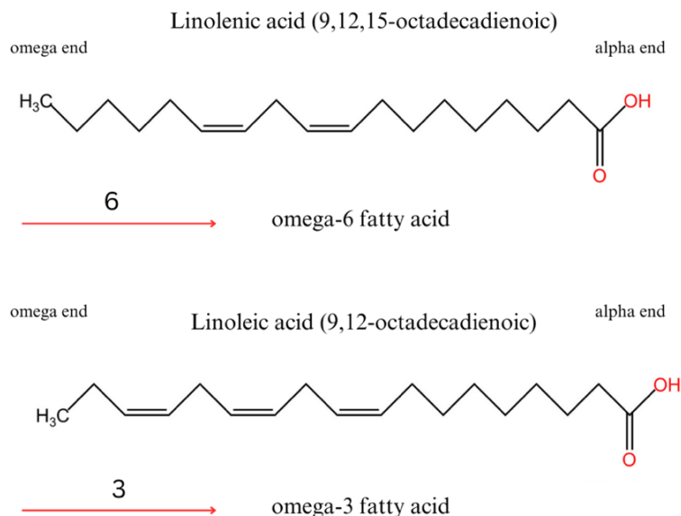
Figure 2. Structure of omega-3 and omega-6 fatty acids
